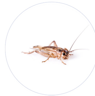
KILGID Acheta domesticus
